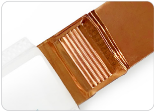
Sonic welded to bus bar
